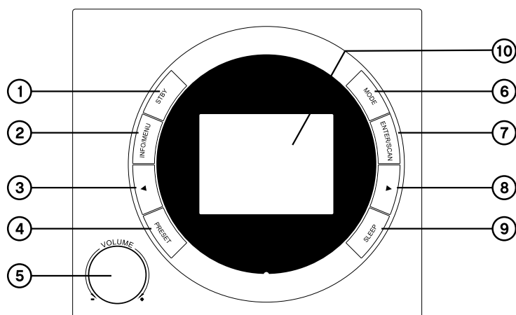
front panel
